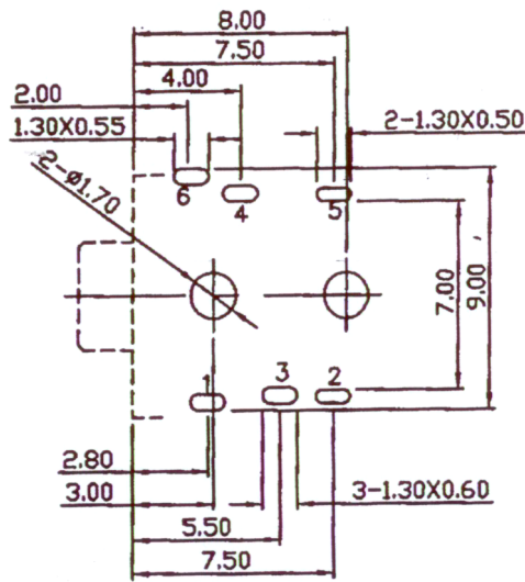
Pin Hole Layout (Jack Bottom View)
