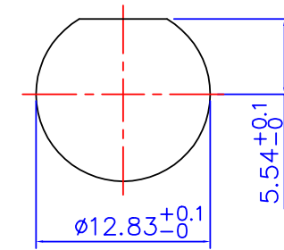
RECOMMENDED MOUNTING HOLE MAXIMUM PANEL THICKNESS: 5.5MM
