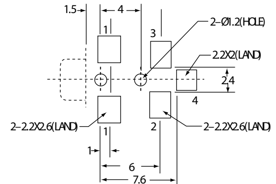
PAD LAYOUT
