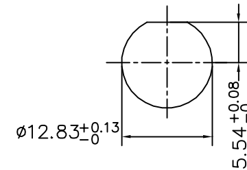
RECOMMENDED MOUNTING HOLE MAXIMUM PANEL THICKNESS: 5.5MM
