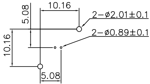
RECOMMENDED PC BOARD LAYOUT WITHOUT MOUNTING POSTS
